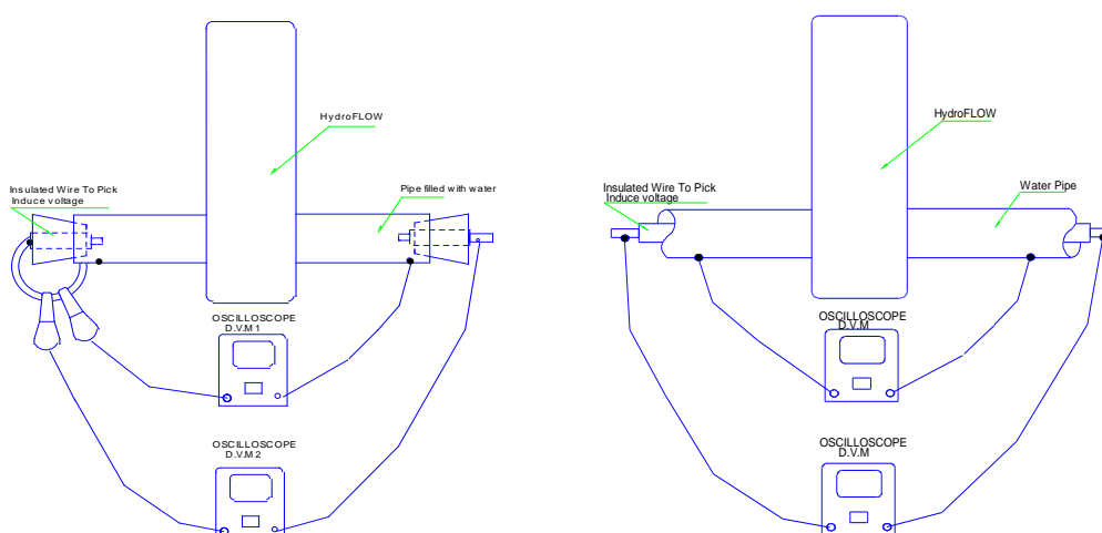
Figure 7: Testing on the Hydroflow
