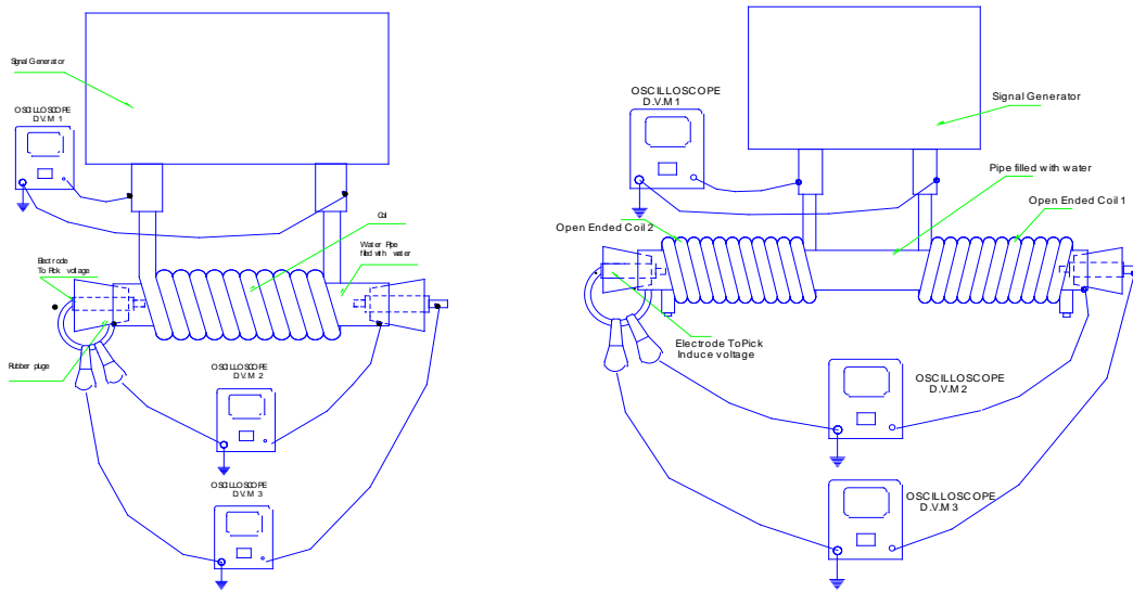
Figure 5: Testing on the single and double coil systems
