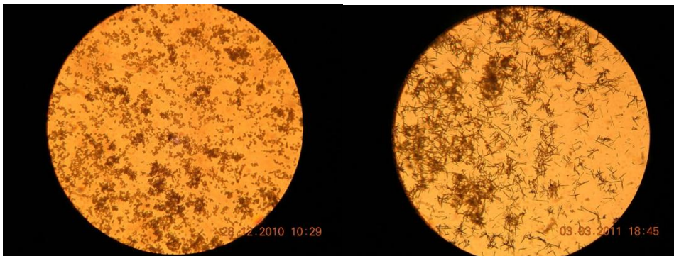
Figure 9: Crystals formed by untreated water (left) and treated water (right)
