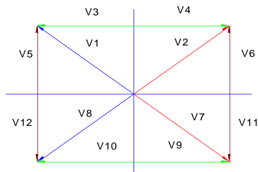
Figure 3: Vector summation of the magnetic field lines produced by an electromagnet.
